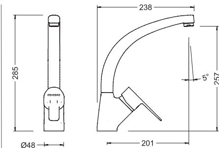
Grifo de cocina monomando caño fundido K8 K8 Single lever sink mixer casted spout
