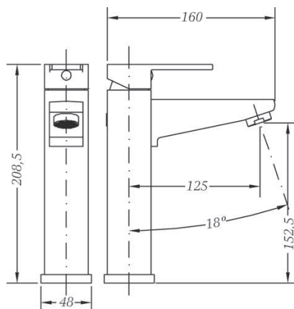
Monomando de lavabo medio alto Medium height single lever wash-basin mixer
