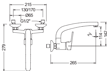
Grifo de cocina monomando mural 15 cm Wall single-lever sink mixer 15 cm
