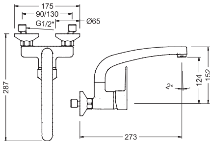
Grifo de cocina monomando mural 11 cm Wall single lever sink mixer 11 cm
